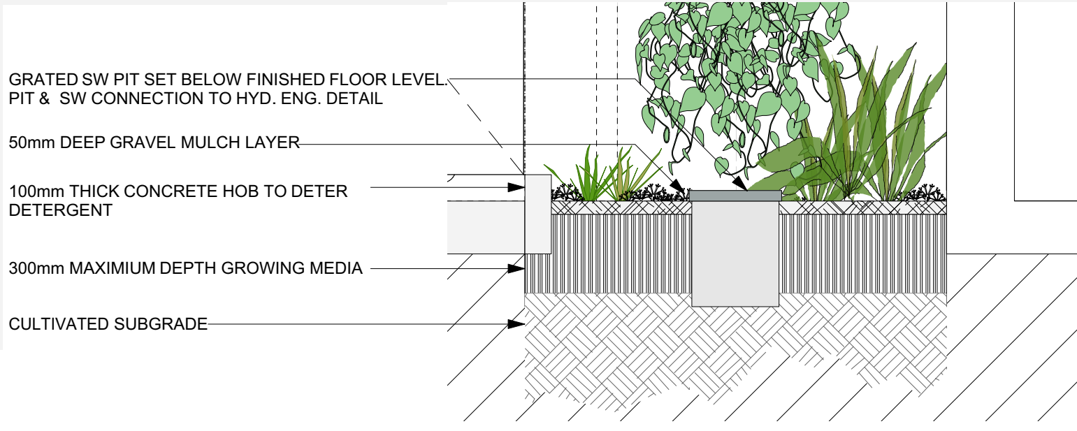
D02 TYPICAL ON GRADE PLANTER SOIL & DRAINAGE PROFILE 1:20 @A1
